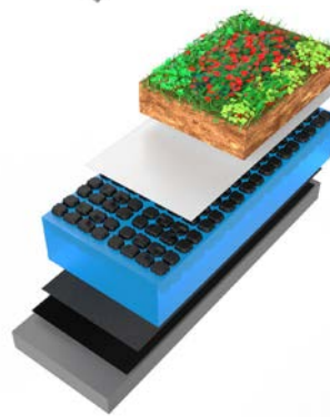
Blue roof extensive - 120 Blue roof
