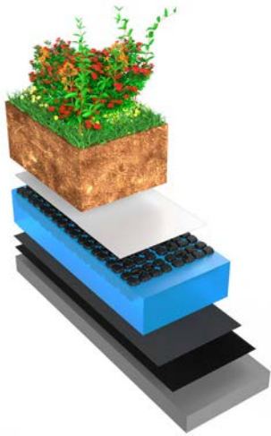
Blue roof semi-intensive 120 Blue roof
