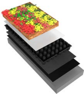
Extensive - 25 LowC Extensive green roof runoff reduction
