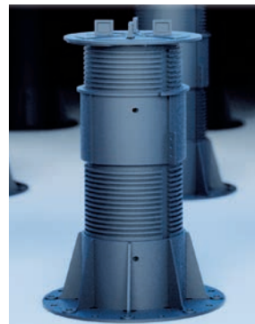
Yggdrasil height adjustable pedestal 19-25 / 28-36 / 36-51 / 52-82 / 82-135 / 133-225 mm
