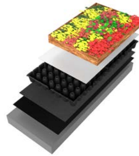
Extensive - 25 FLL Extensive green roof
