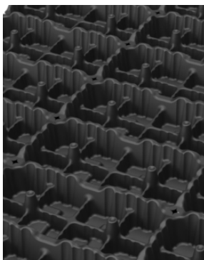
QSDrain-60 Free Without water storage for road traffic
