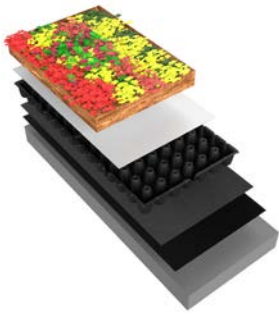
Extensive - 20 Extensive green roof
