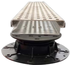
Height adjustment with Yggdrasil pedestal
