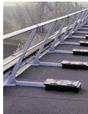
Railing - 30 degree EN 14122
