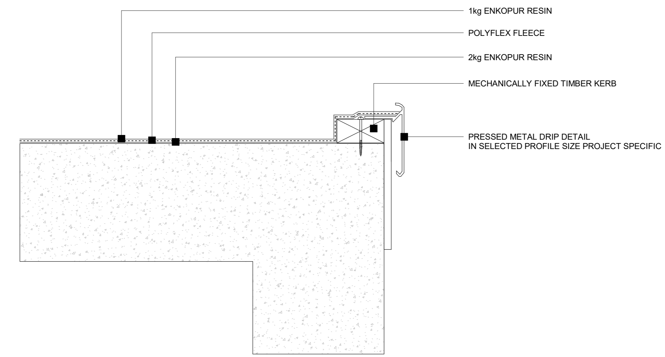
17 Enke - Concrete Deck - Water check detail 1 : 5
