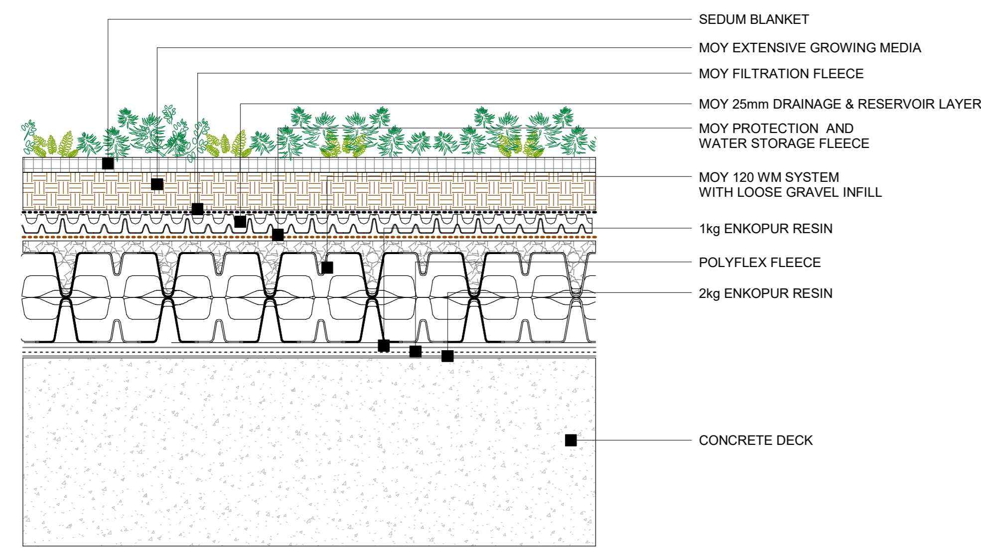
13 Enke - Concrete Deck - Green roof assembly 1 : 5
