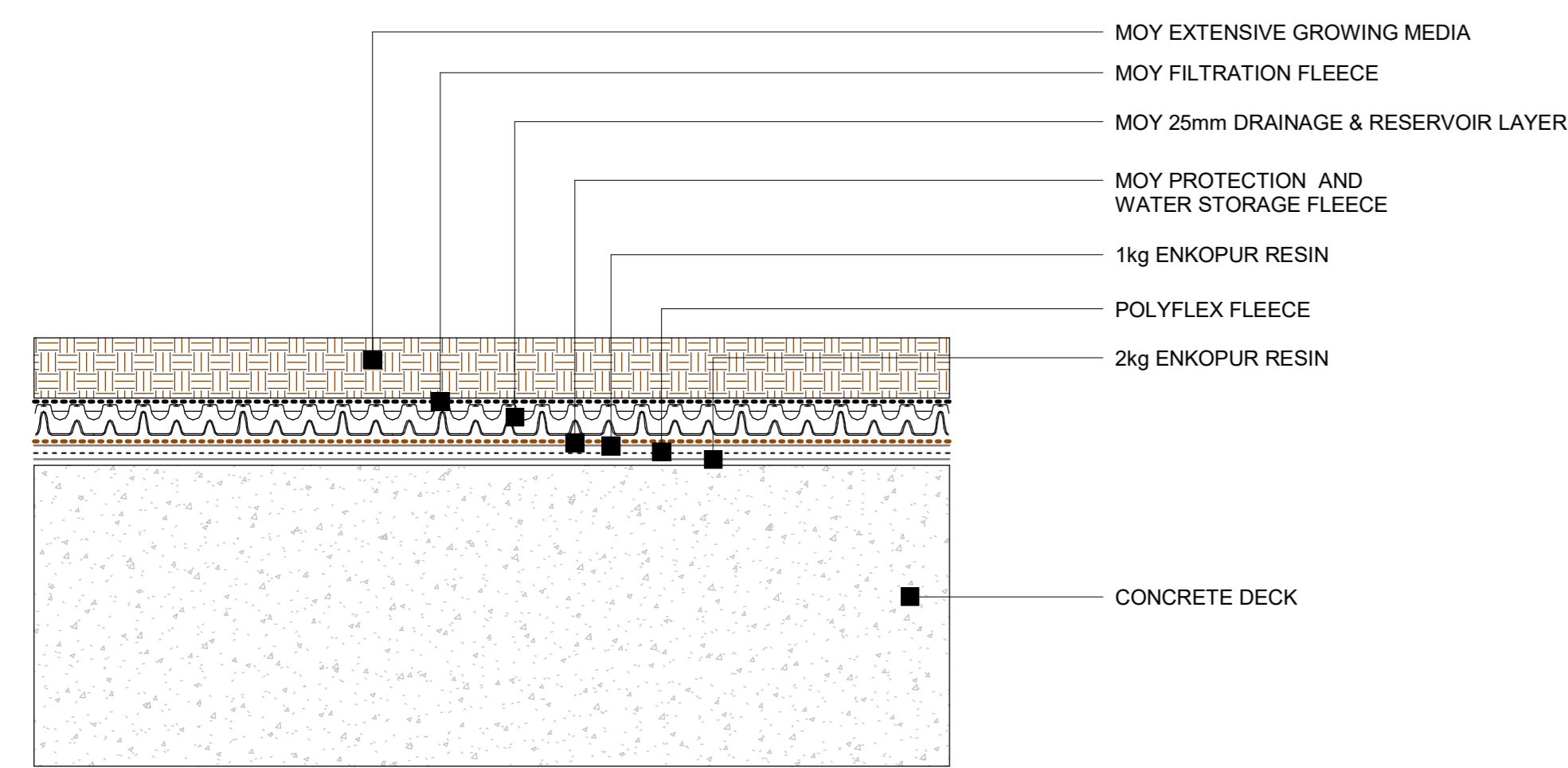
14 Enke - Concrete Deck - Blue roof assembly 1 : 5
