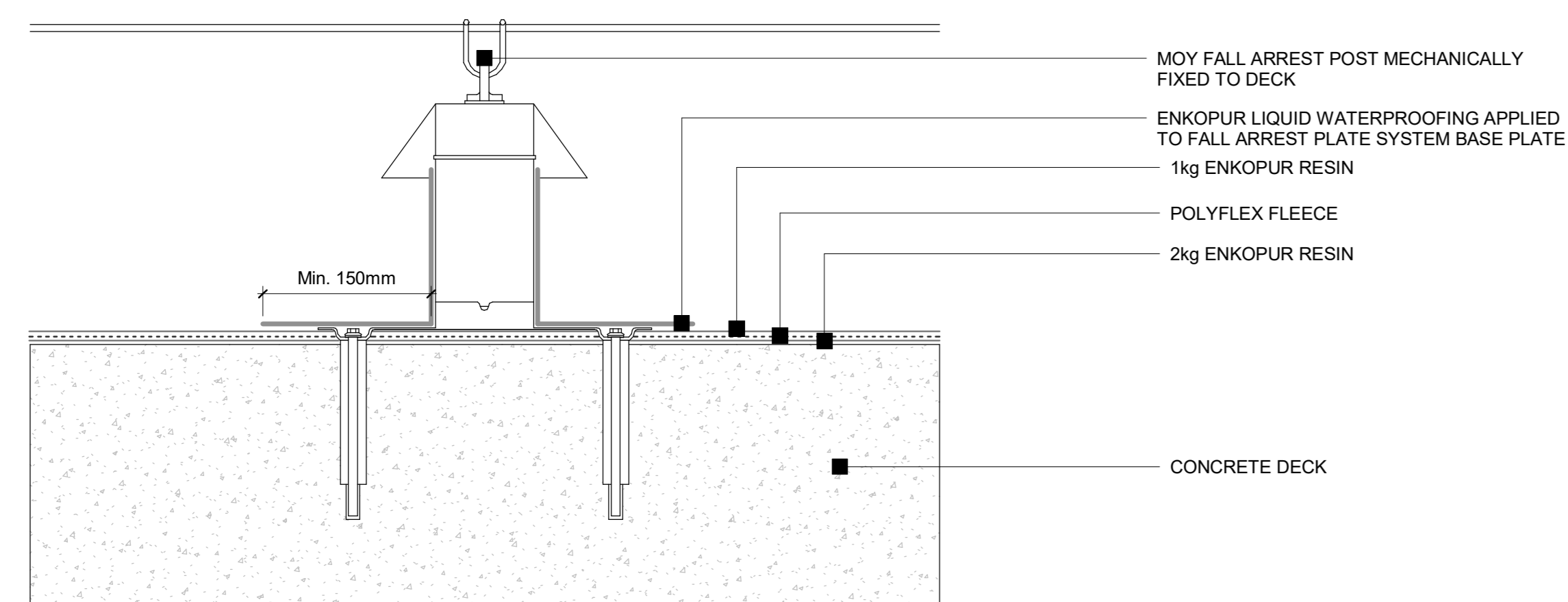
15 Enke - Concrete Deck - Brown roof assembly 1 : 5
