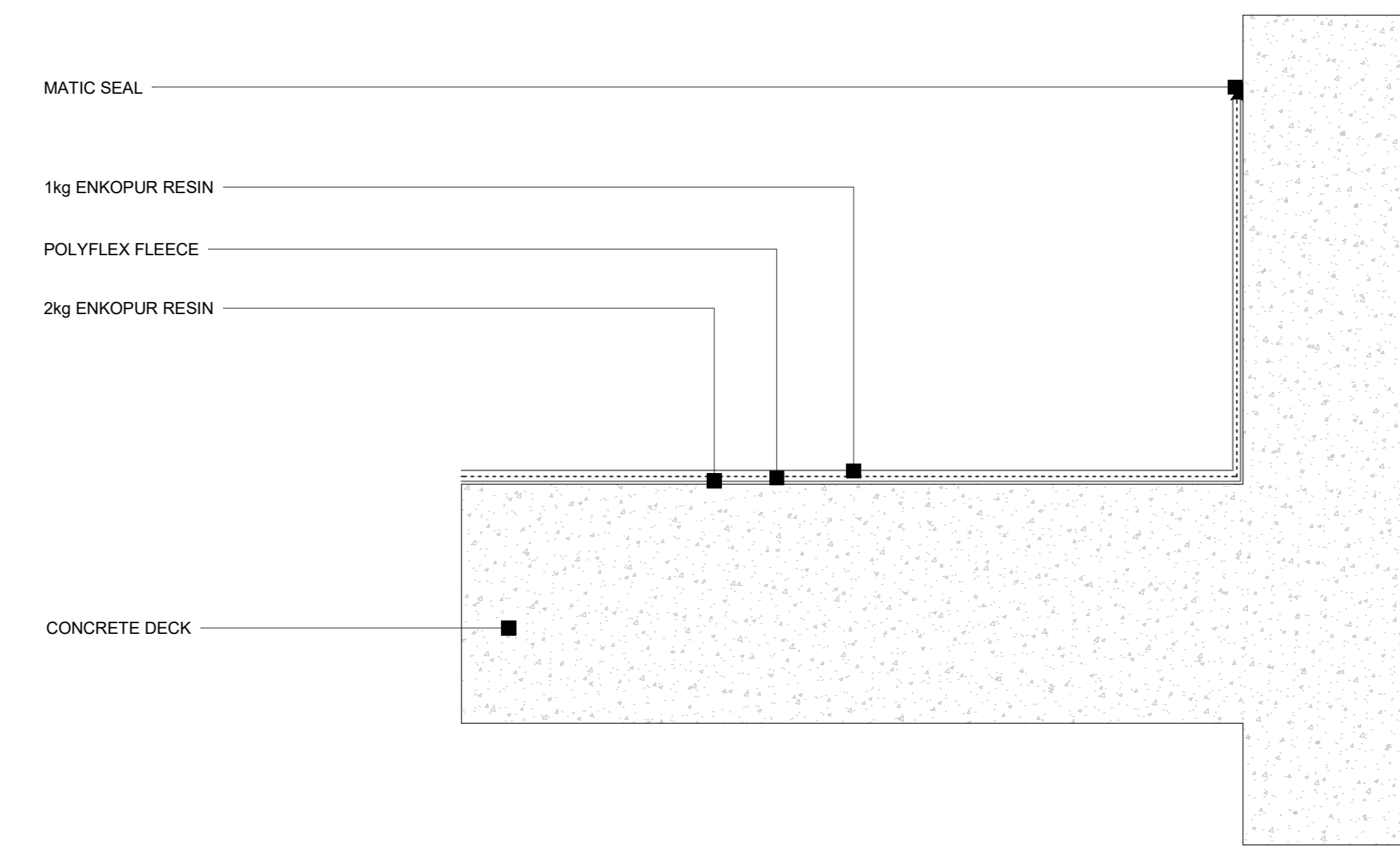
18 Enke - Concrete Deck - Self termination detail 1 : 5
