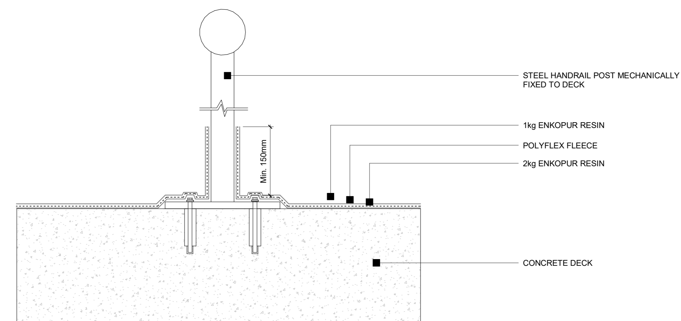
19 Enke - Concrete Deck - Termination to handrail detail 1 : 5
