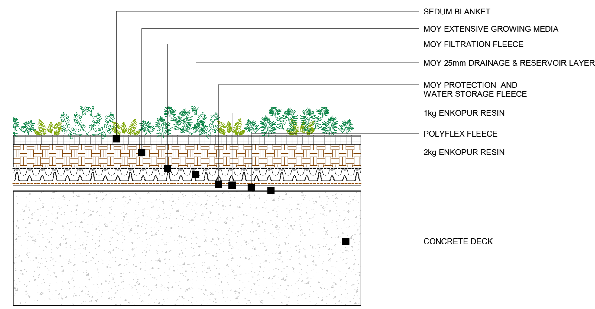
13 Enke - Concrete Deck - Green roof assembly 1 : 5
