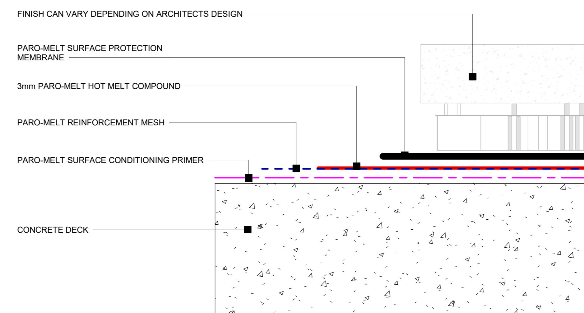
5 Paro-melt System Elements 1:2
