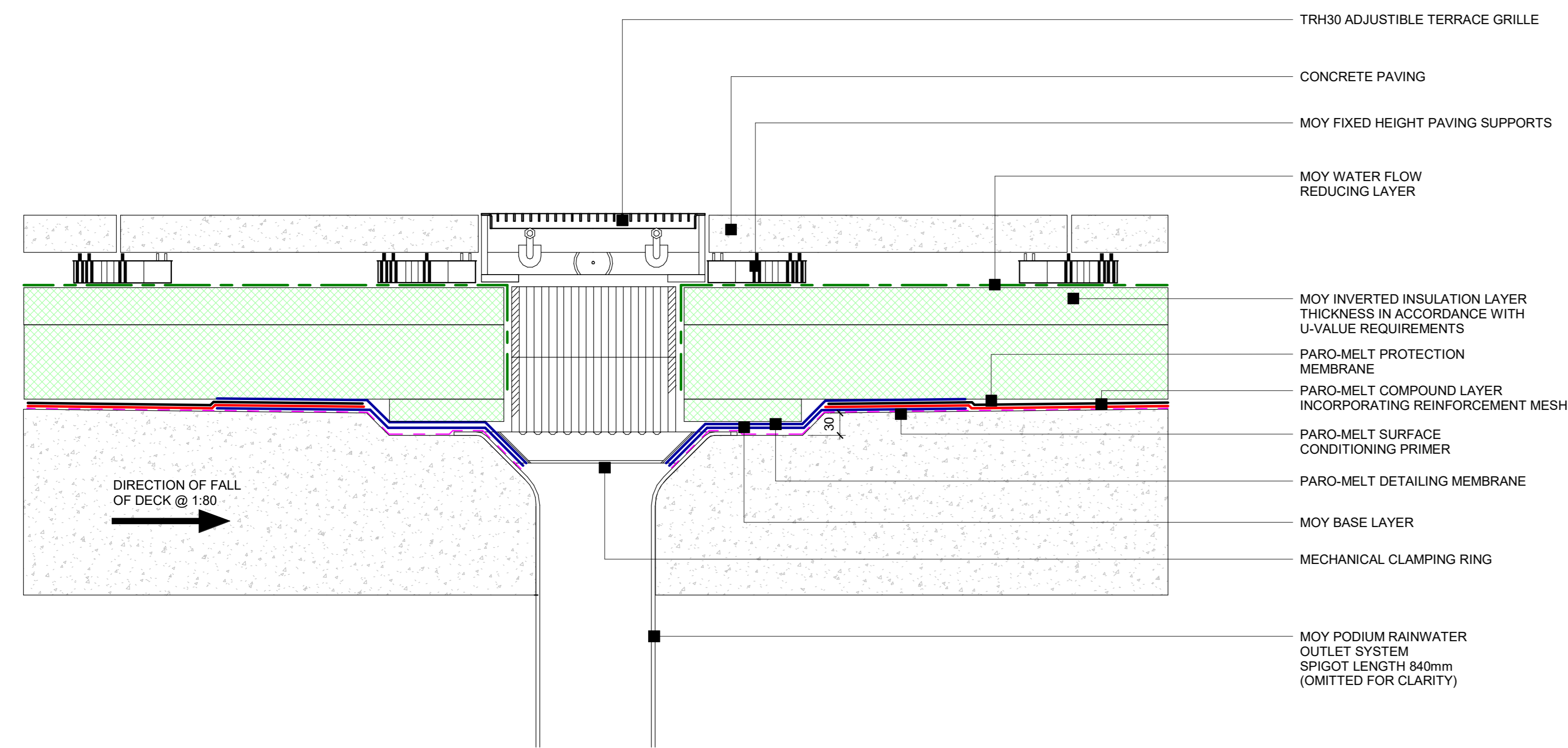
1 Paro-melt System - Vertical Spigot Gravity Rainwater Outlet Detail 1:5
