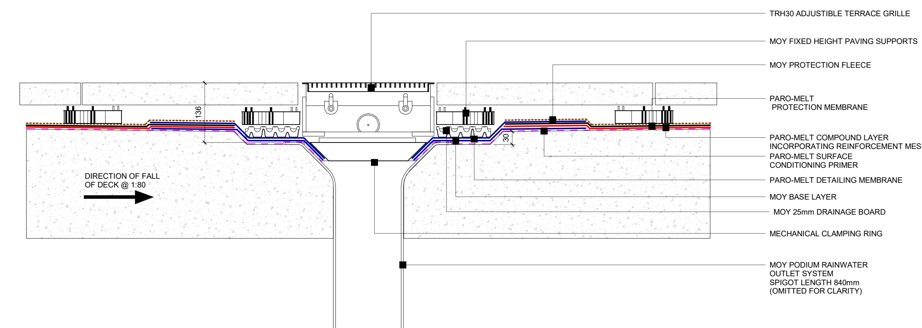
2 Paro-melt System - Outlet Detail (Cold deck) 1:5
