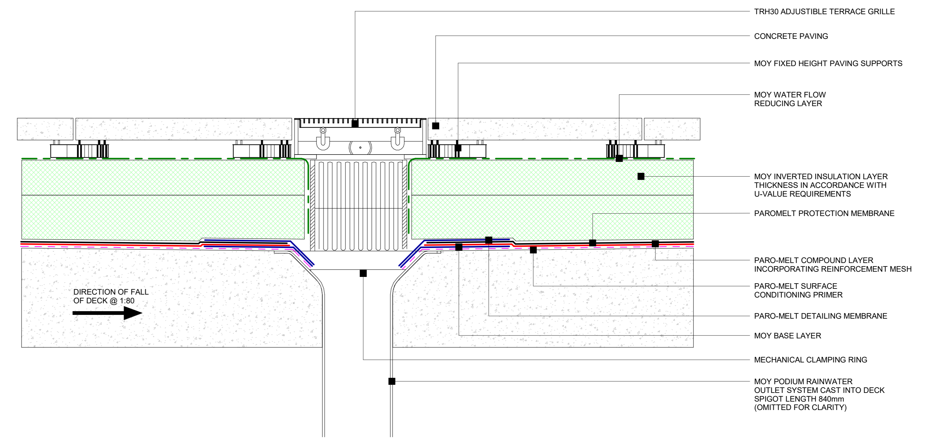
3 Paro-melt System - Outlet Detail (No Sump) 1:5
