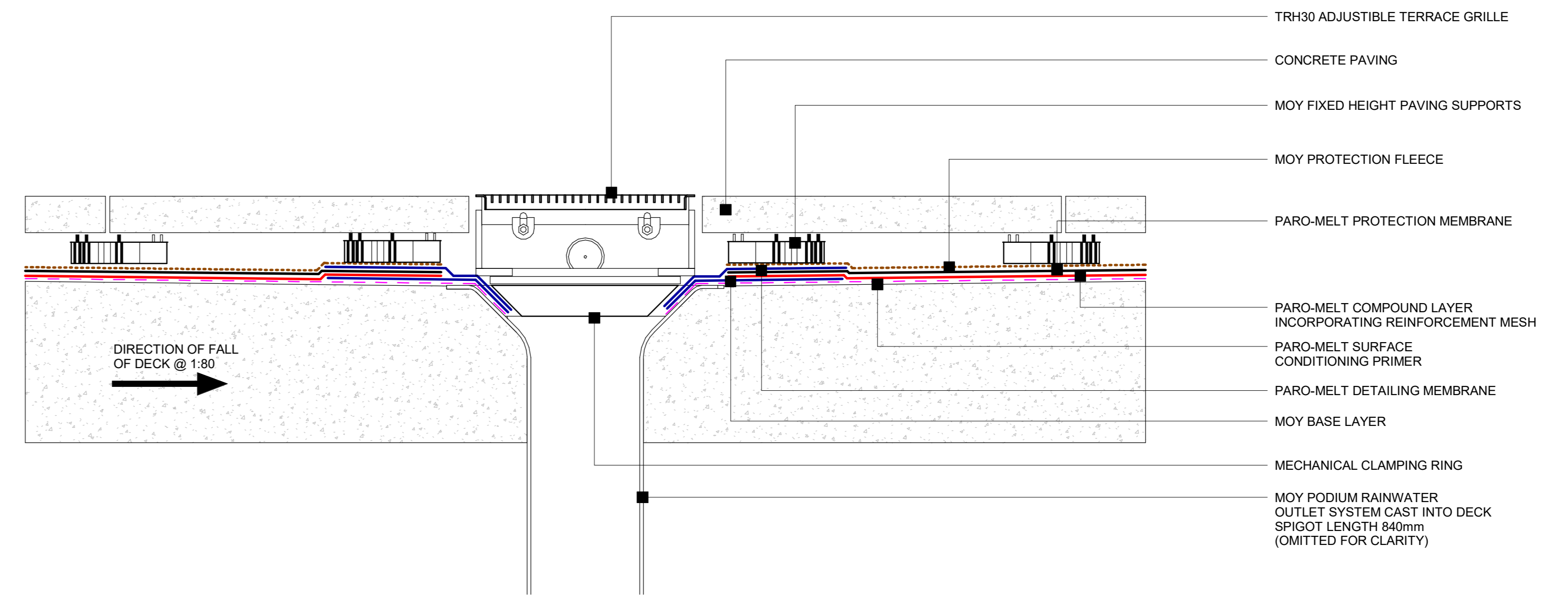
4 Paro-melt System - Outlet Detail (No Sump / Cold deck) 1:5
