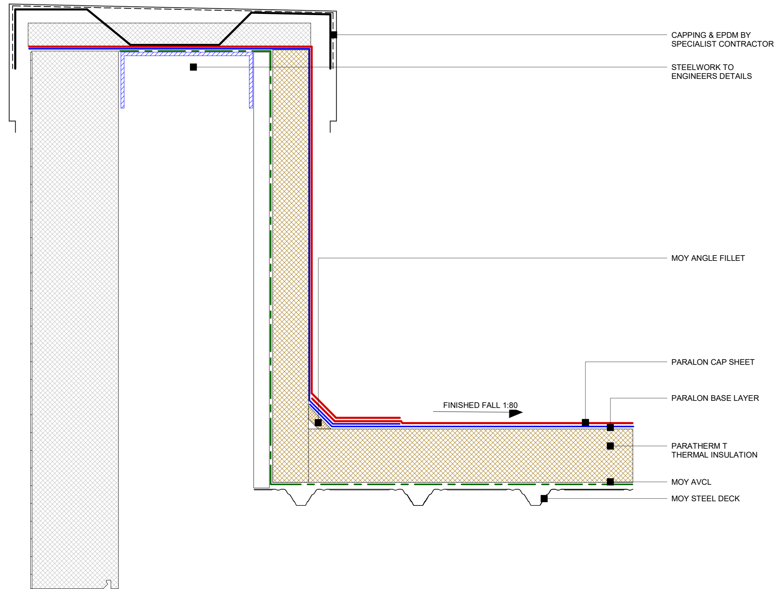
1 Paralon Steel Deck - Mechanically Attached Method of Application 1:5
