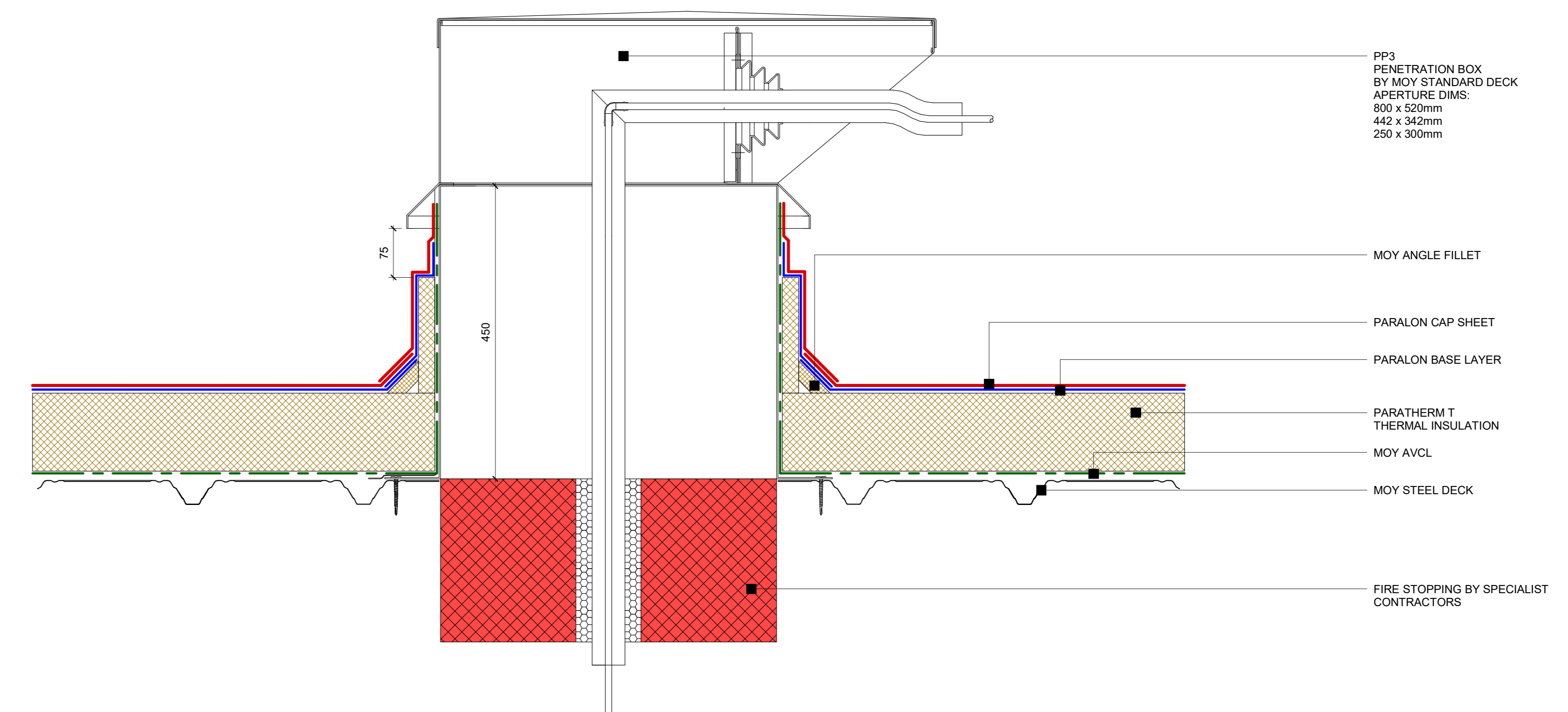
6 Paralon Steel Deck - PP3 Cable Penetration Box Detail 1:5
