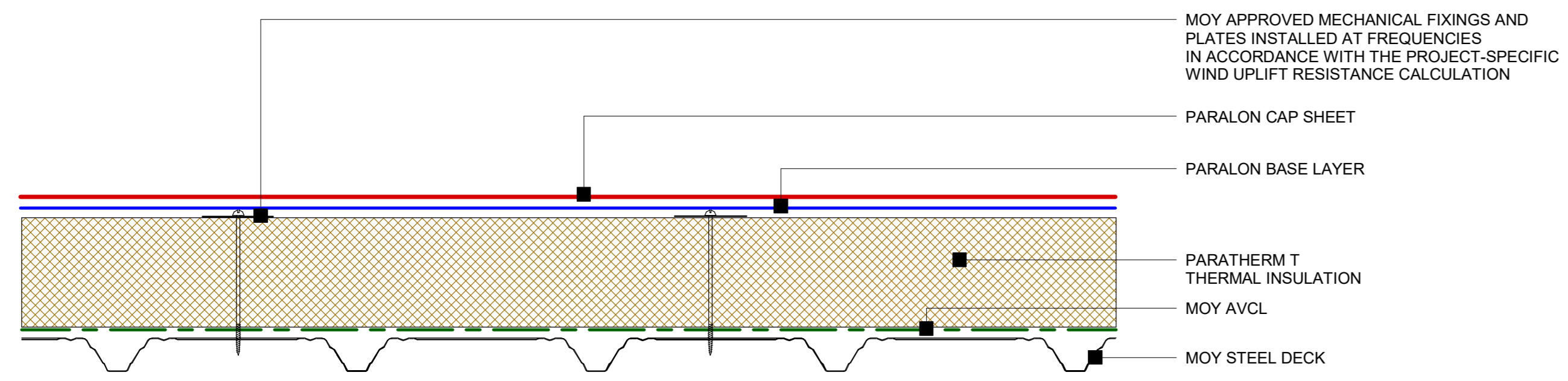
1 Paralon Steel Deck - Mechanically Attached Method of Application 1:5
