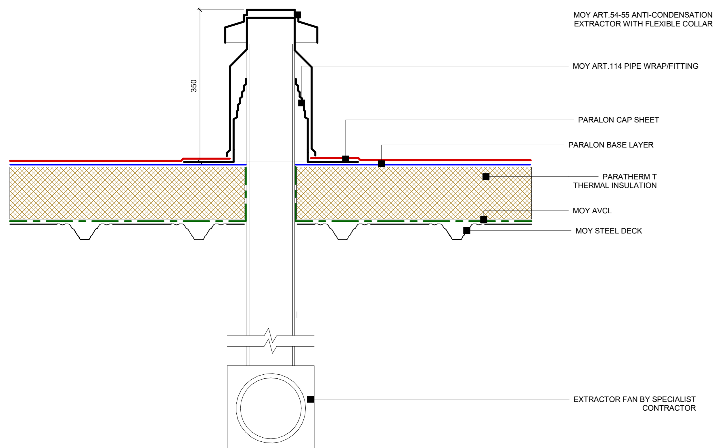
3 Paralon Steel Deck - Vent Pipe Detail 1:5
