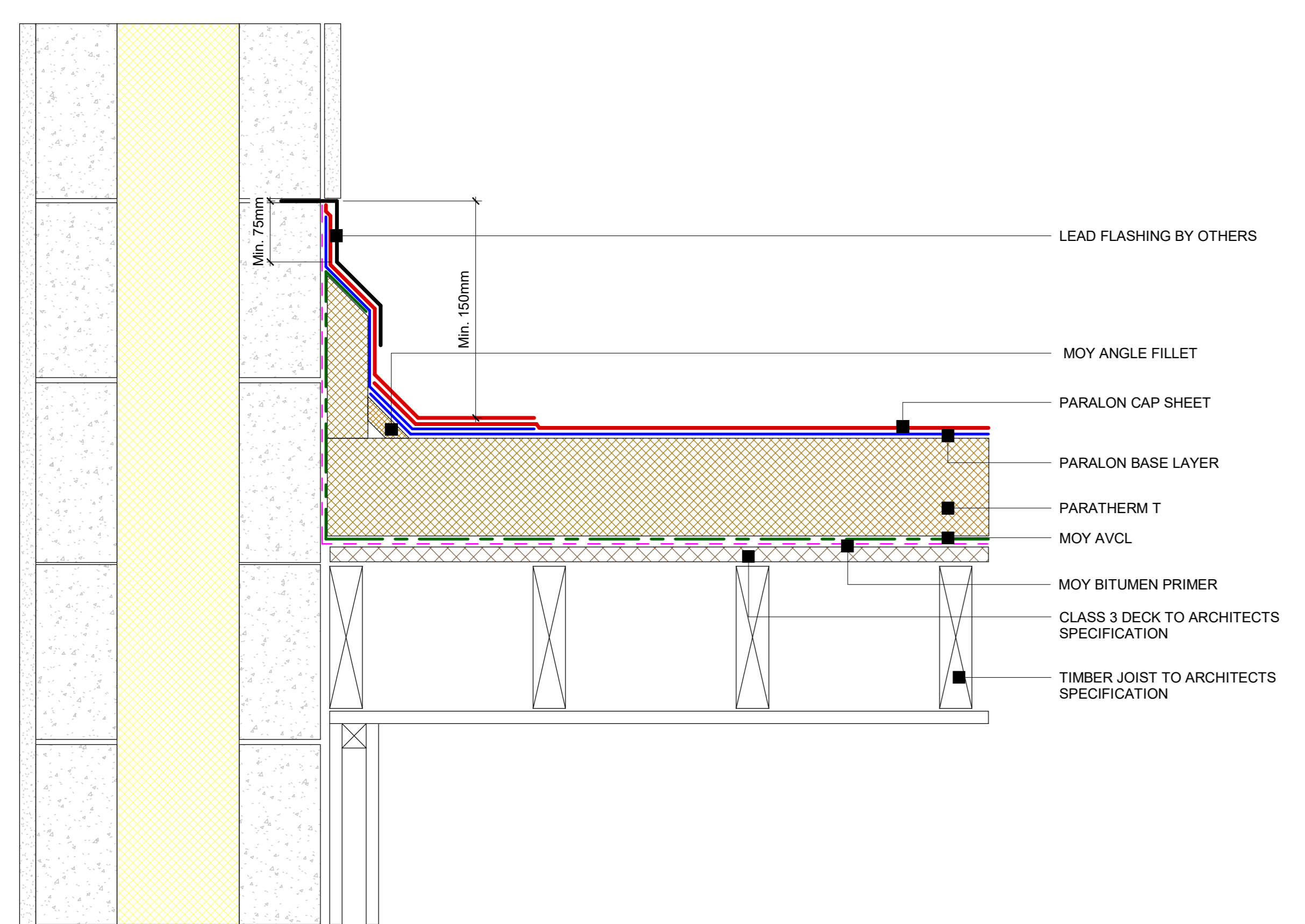
8 Paralon Timber Deck - Masonry Upstand Detail 1:5
