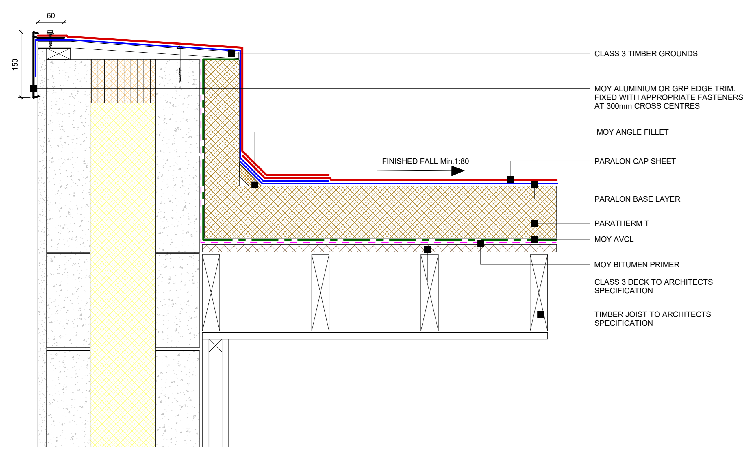
9 Paralon Timber Deck - Parapet Detail (Moy Aluminium or GRP Edge Trim) 1:5
