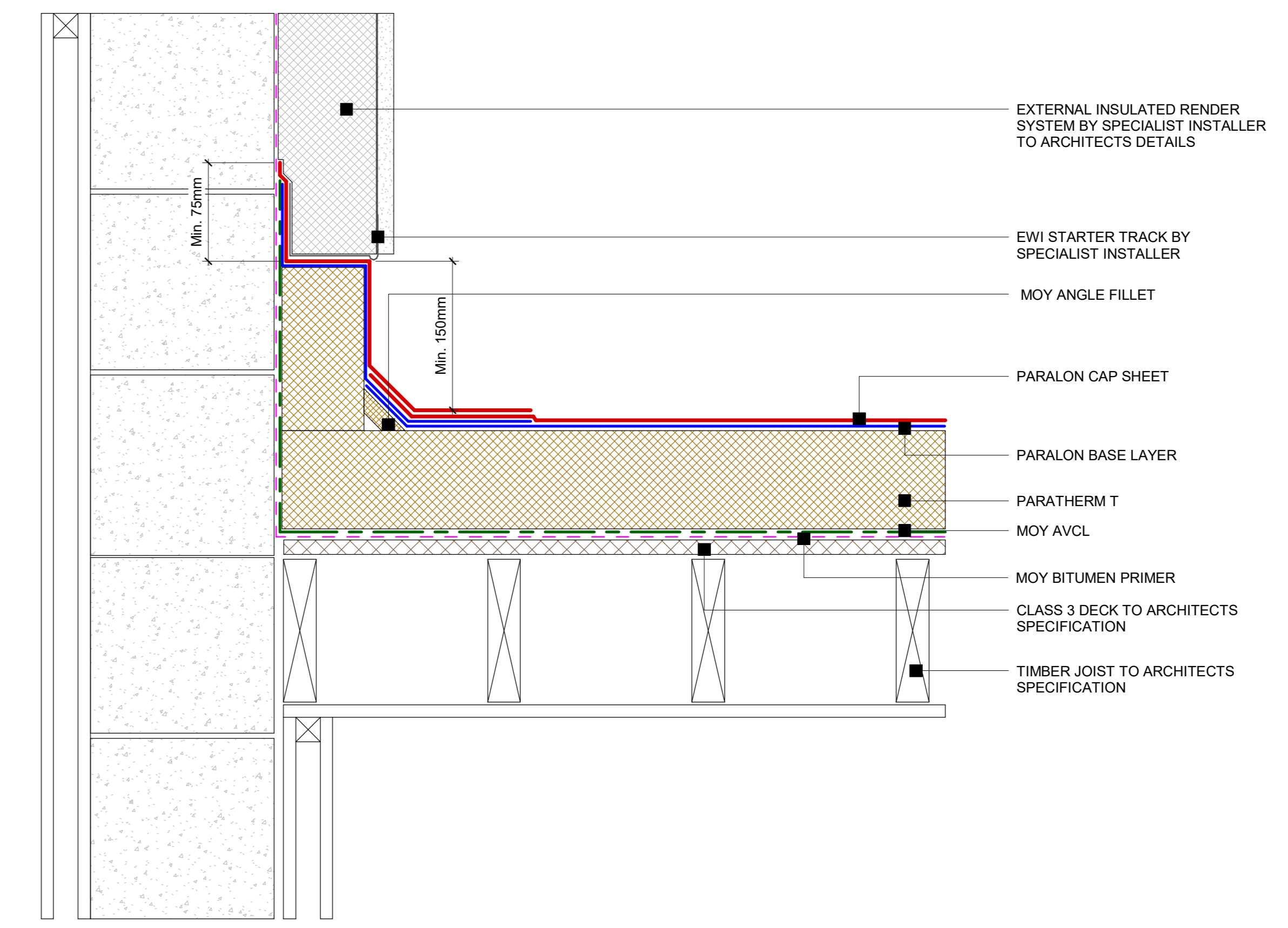
10 Paralon Timber Deck - Upstand With External Insulated Render Detail 1:5
