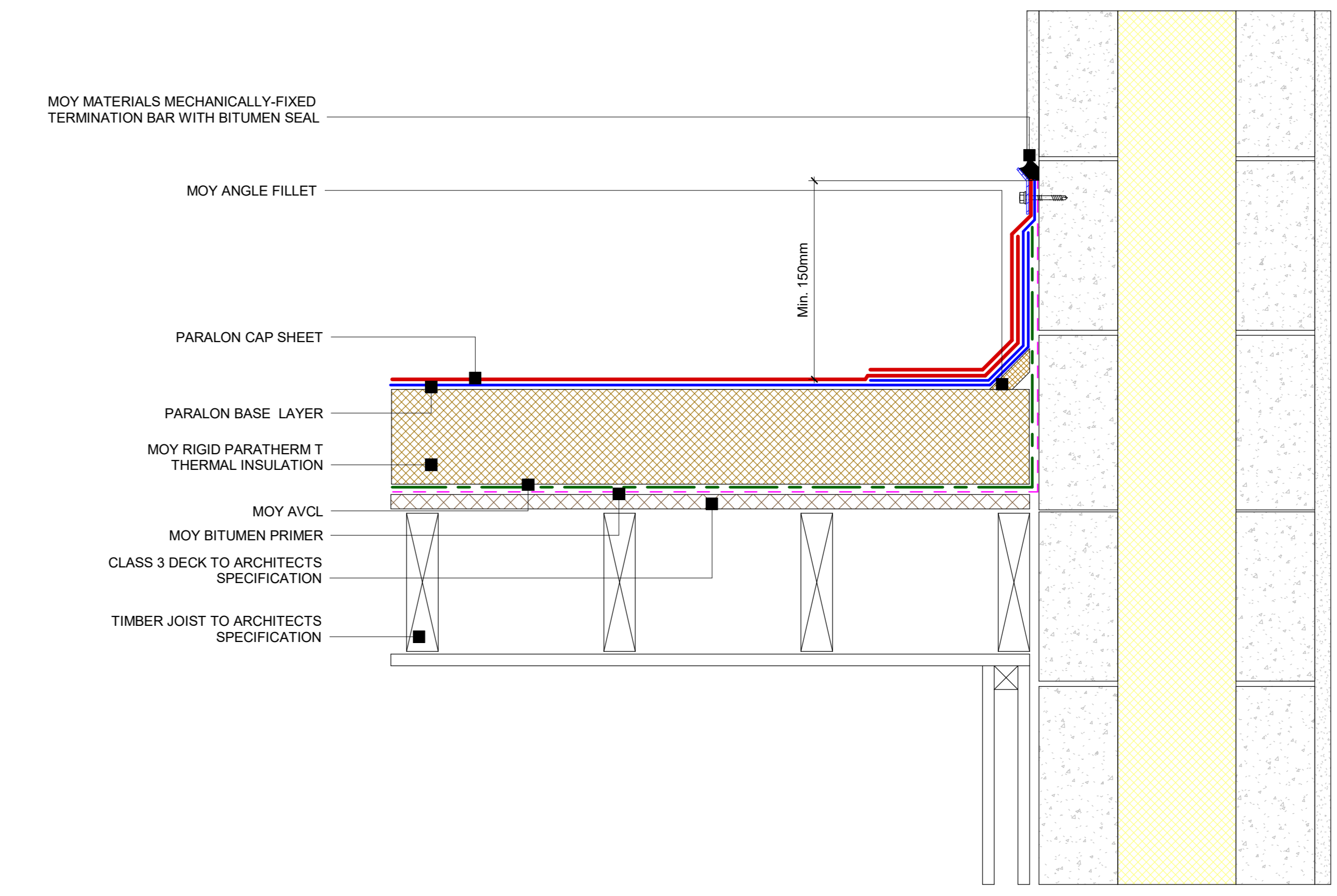
11 Paralon Timber Deck - Termination Bar Detail 1:5
