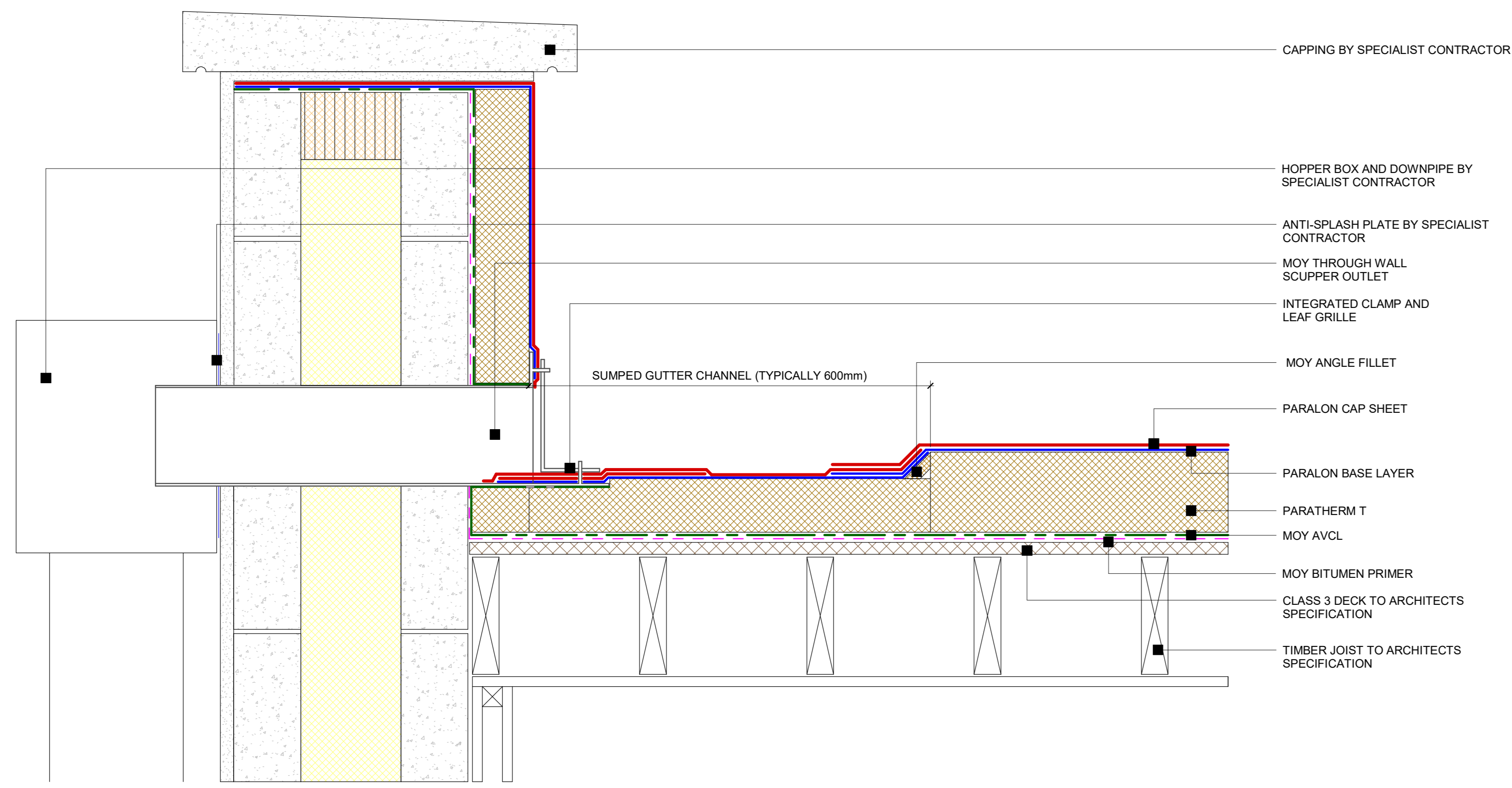
7 Paralon Timber Deck - Parapet Outlet Detail 1:5
