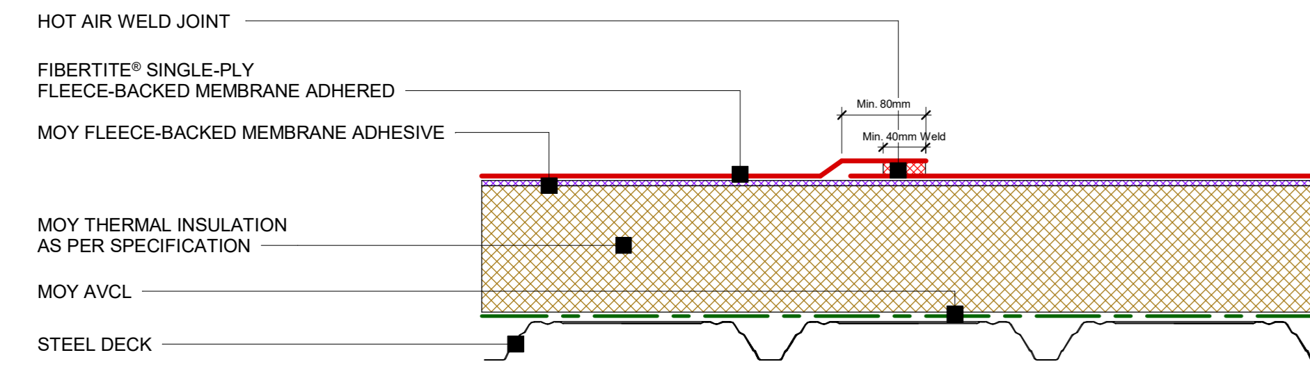
1 FiberTite® - Waterproofing system assembly 1 : 5
