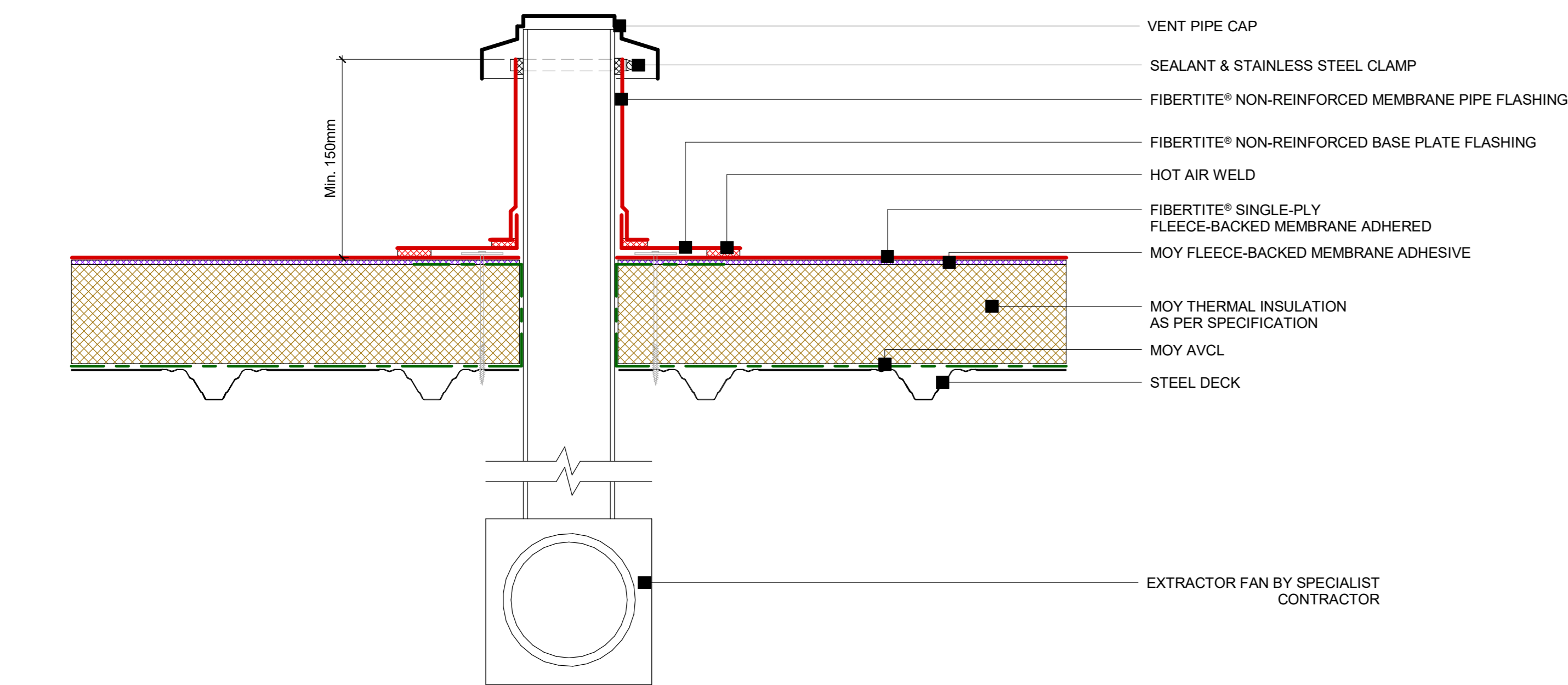
3 FiberTite® - Soil vent pipe detail (Site fabricated) 1 : 5
