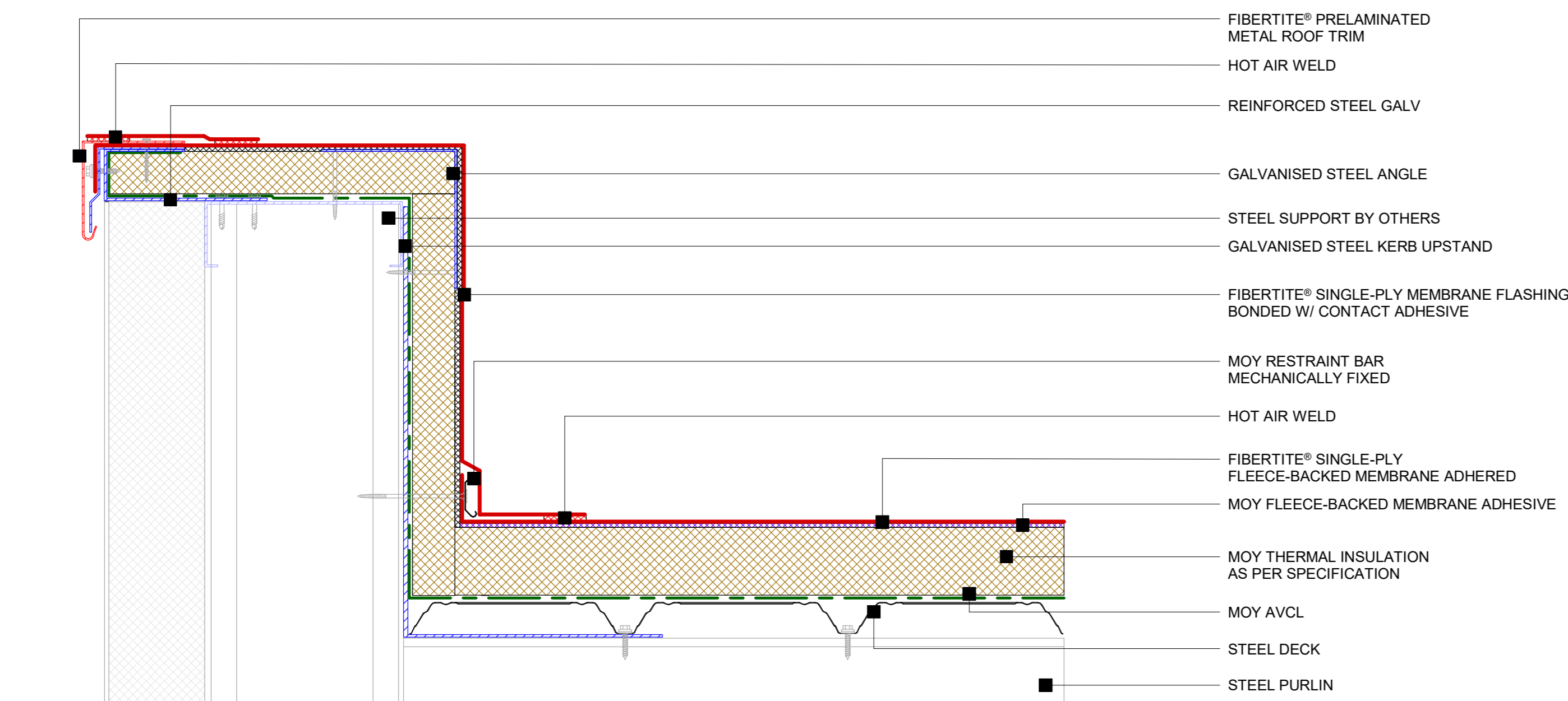
2 FiberTite® - Edge trim upstand detail 1 : 5
