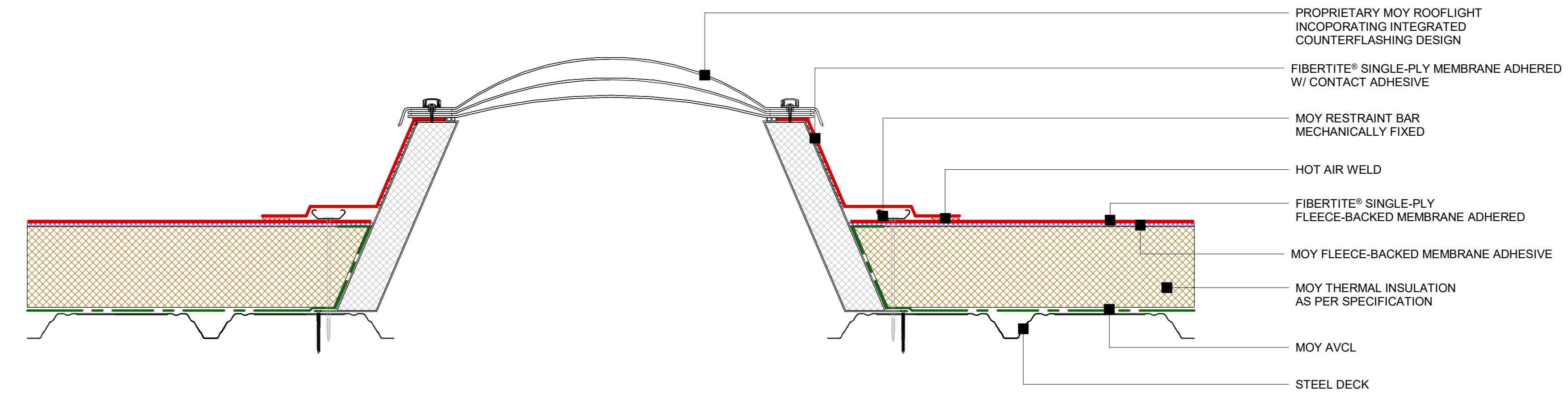
4 FiberTite® - Rooflight detail 1 : 5
