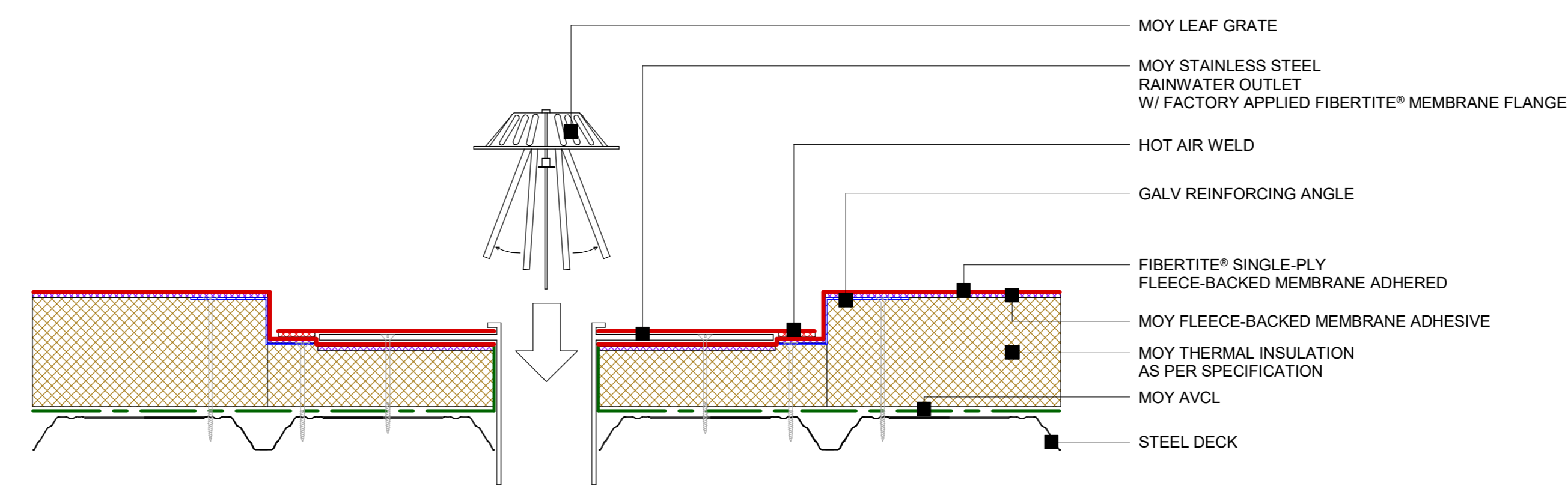
5 FiberTite® - Sumped Rainwater outlet detail 1 : 5
