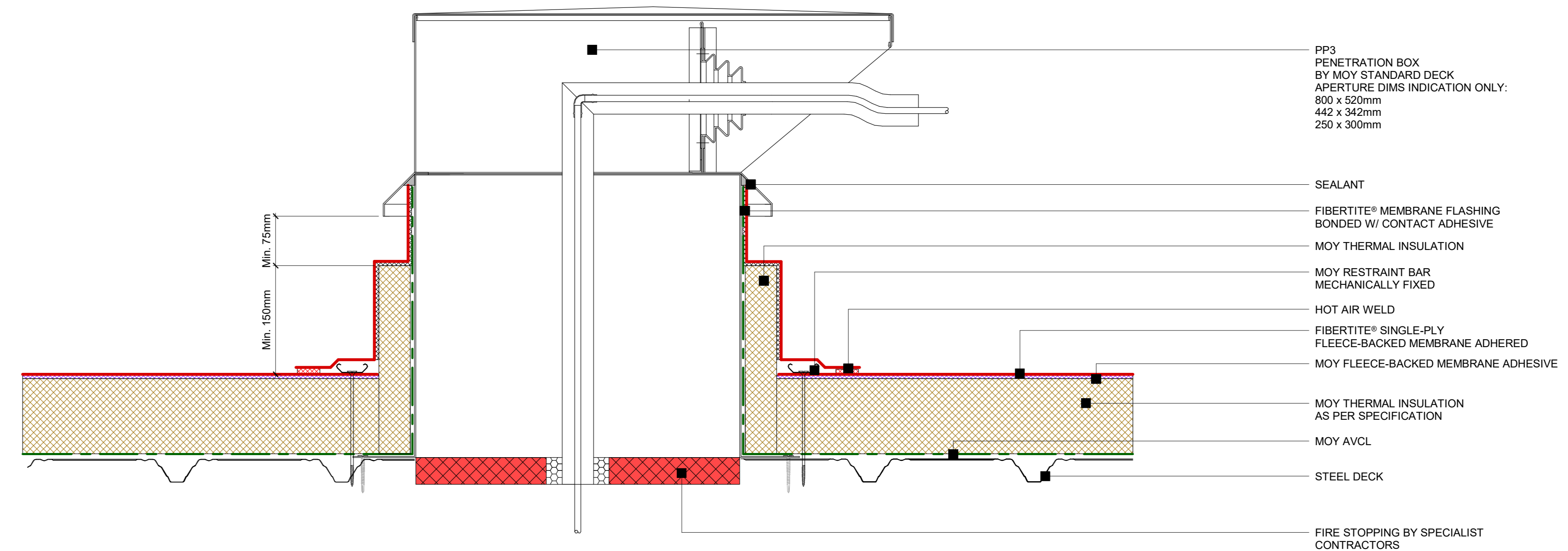
6 FiberTite® - PP3 Cable Penetration Box Detail 1 : 5
