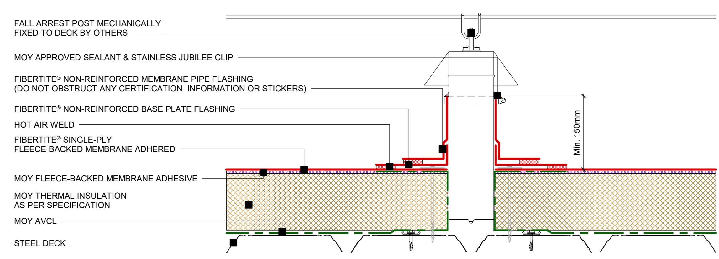
16 FiberTite® - Fall arrest detail 1 : 5
