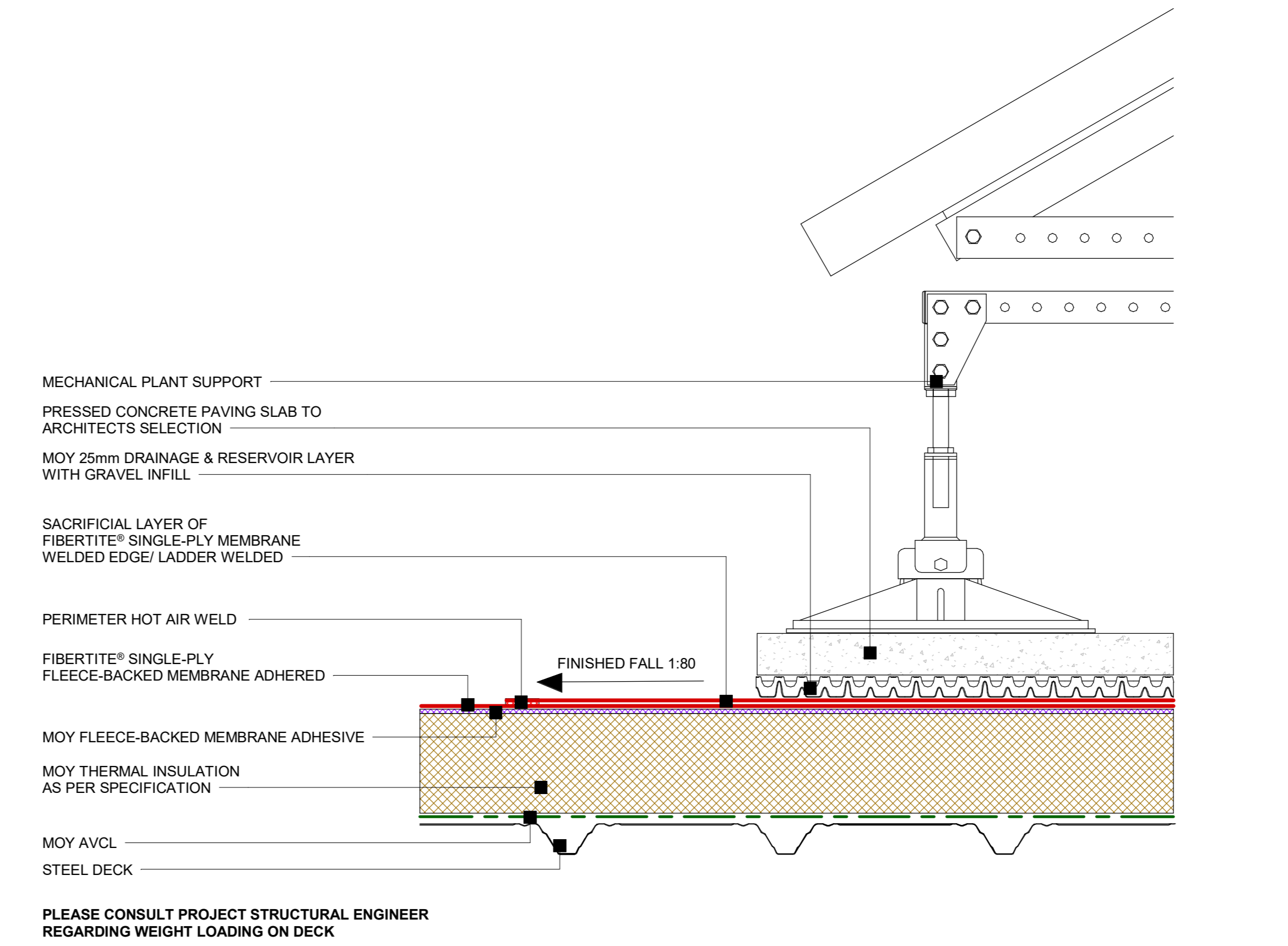
19 FiberTite® - Plant support detail 1 : 5
