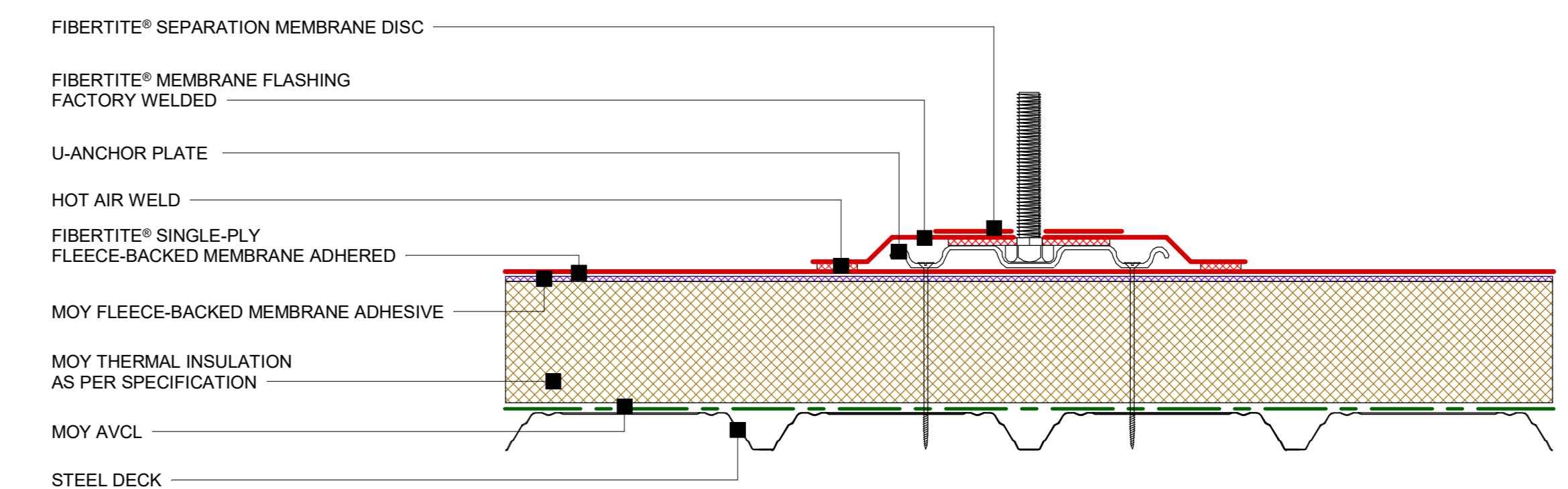
20 FiberTite® - U-Anchor detail 1 : 5
