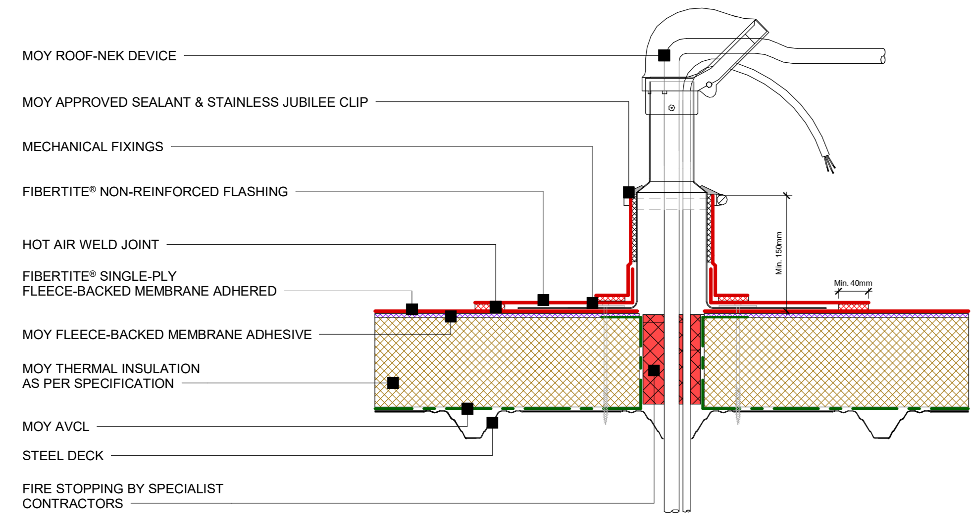
14 FiberTite® - RoofNek cable penetration detail 1 : 5
