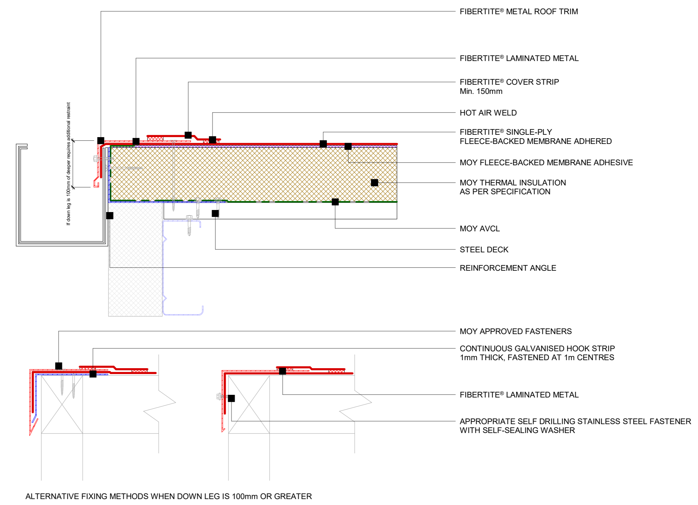
24 FiberTite® - Drip edge to external gutter detail 1 : 5
