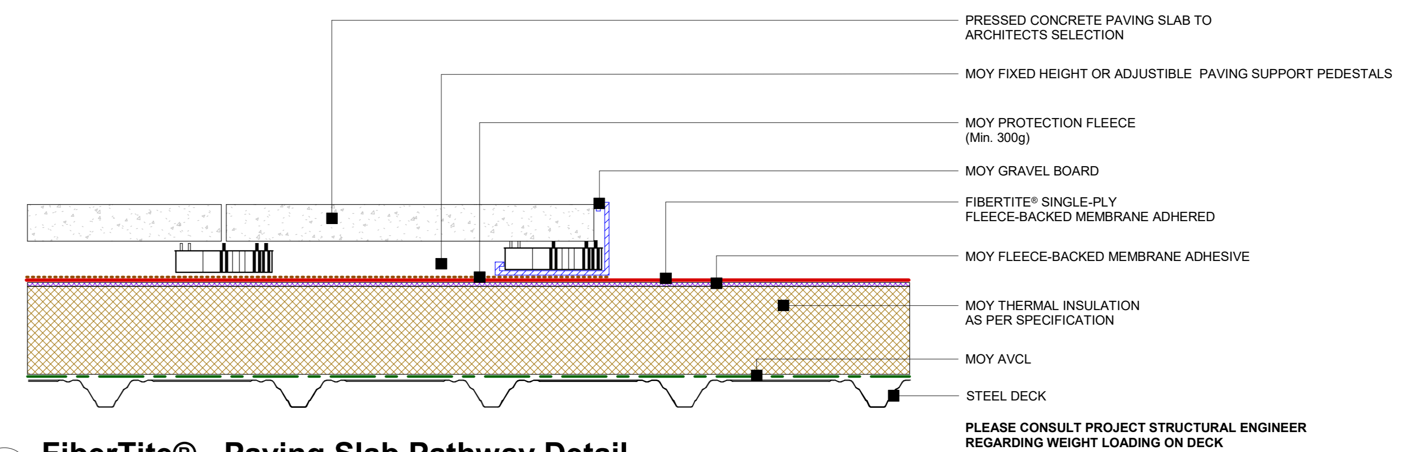
25 FiberTite® - Paving Slab Pathway Detail 1 : 5
