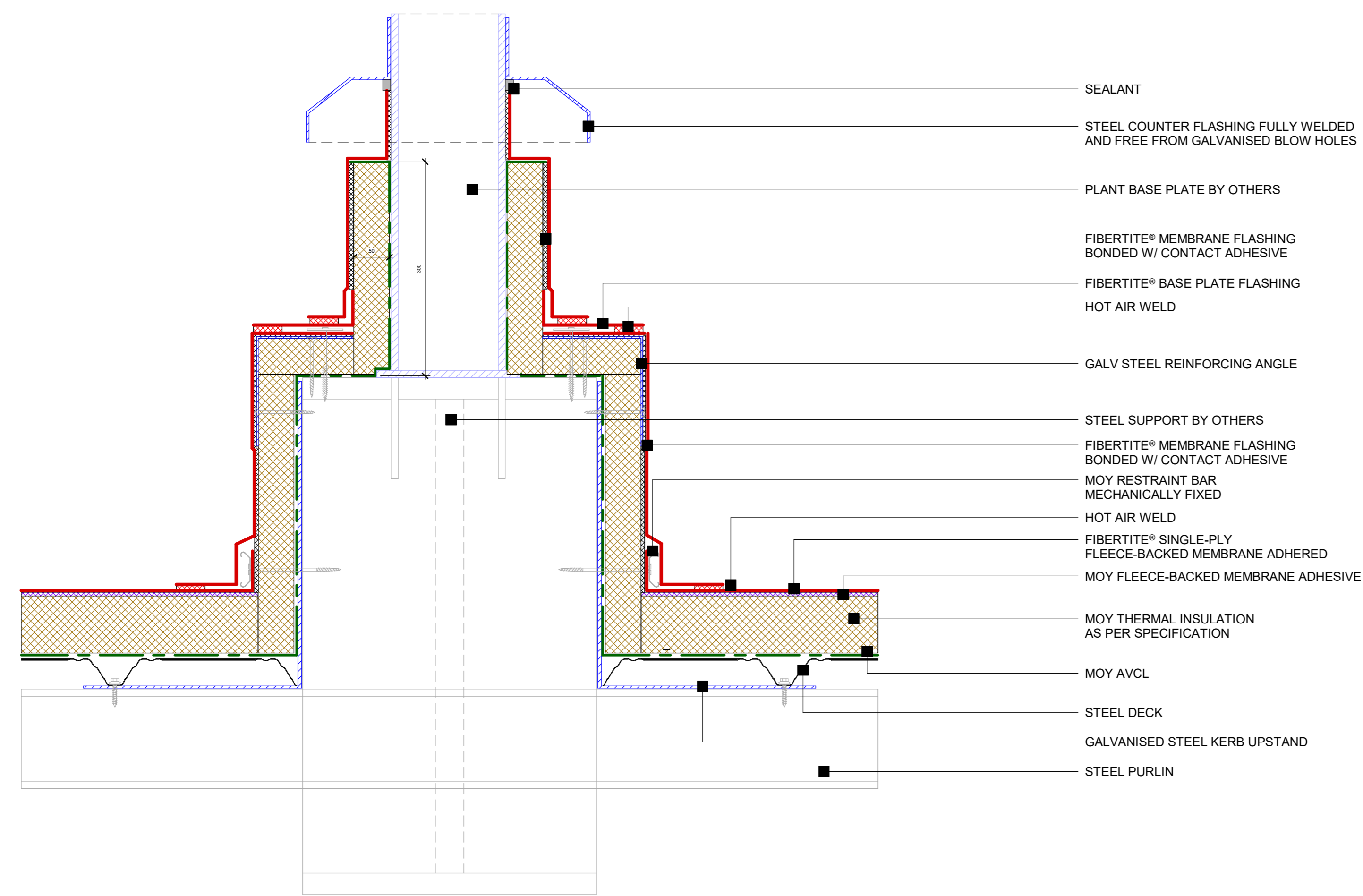
21 FiberTite® - Plant plinth detail 1 : 5
