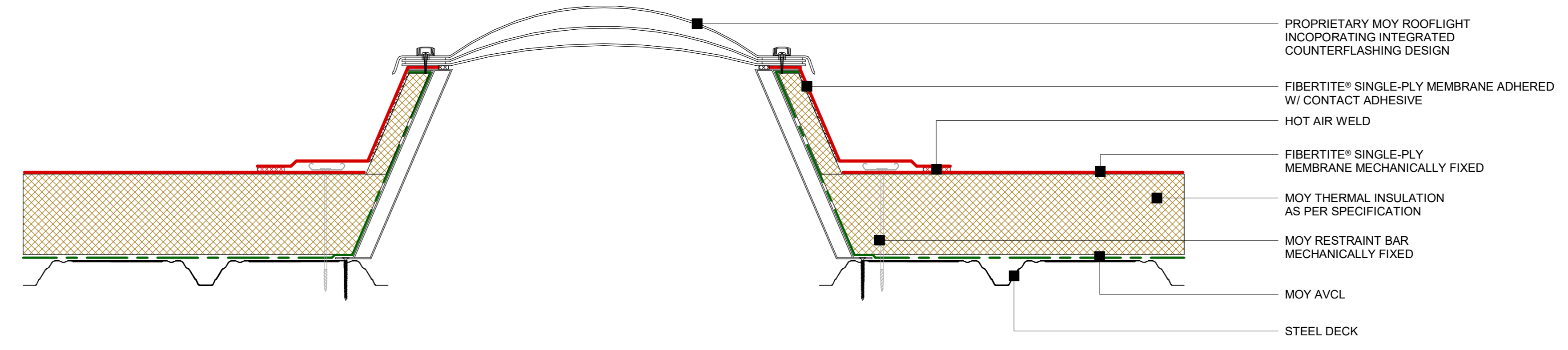
4 Fibertite® - Rooflight detail 1 : 5
