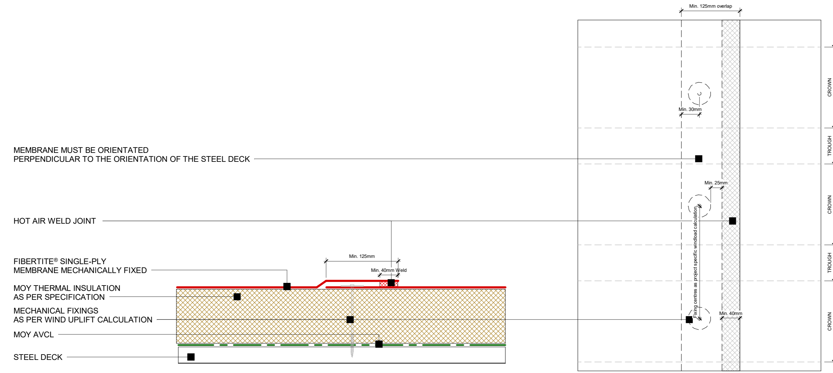
1 Fibertite® - Waterproofing system assembly 1 : 5
