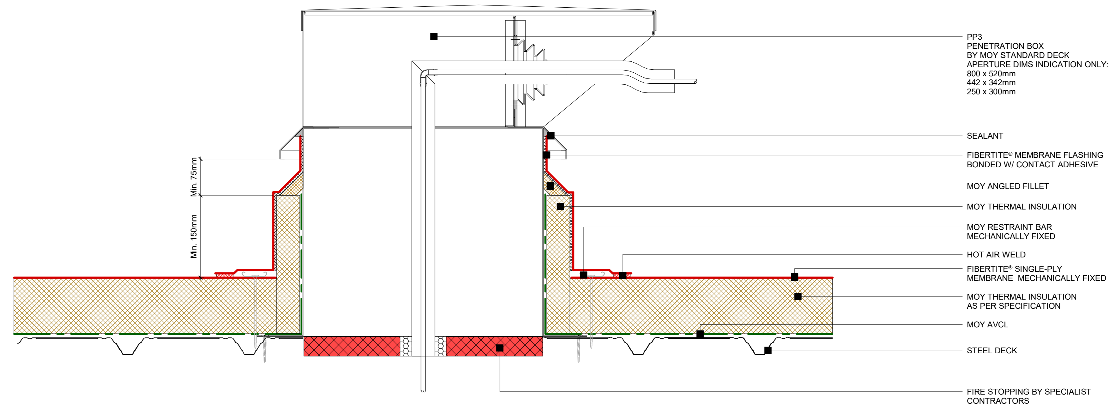
6 Fibertite® - PP3 Cable Penetration Box Detail 1 : 5
