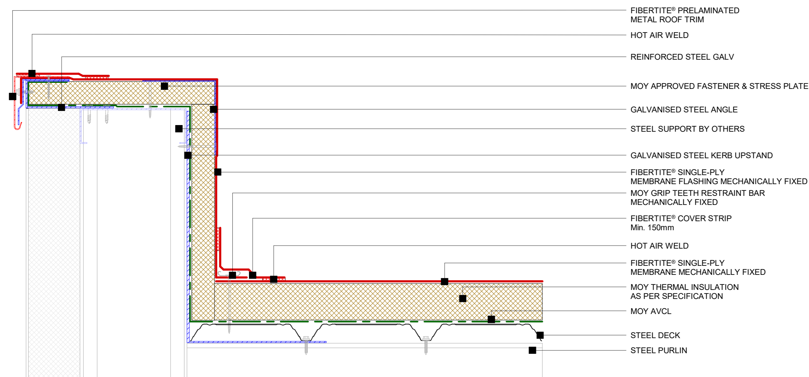
2 Fibertite® - Edge trim upstand detail 1 : 5
