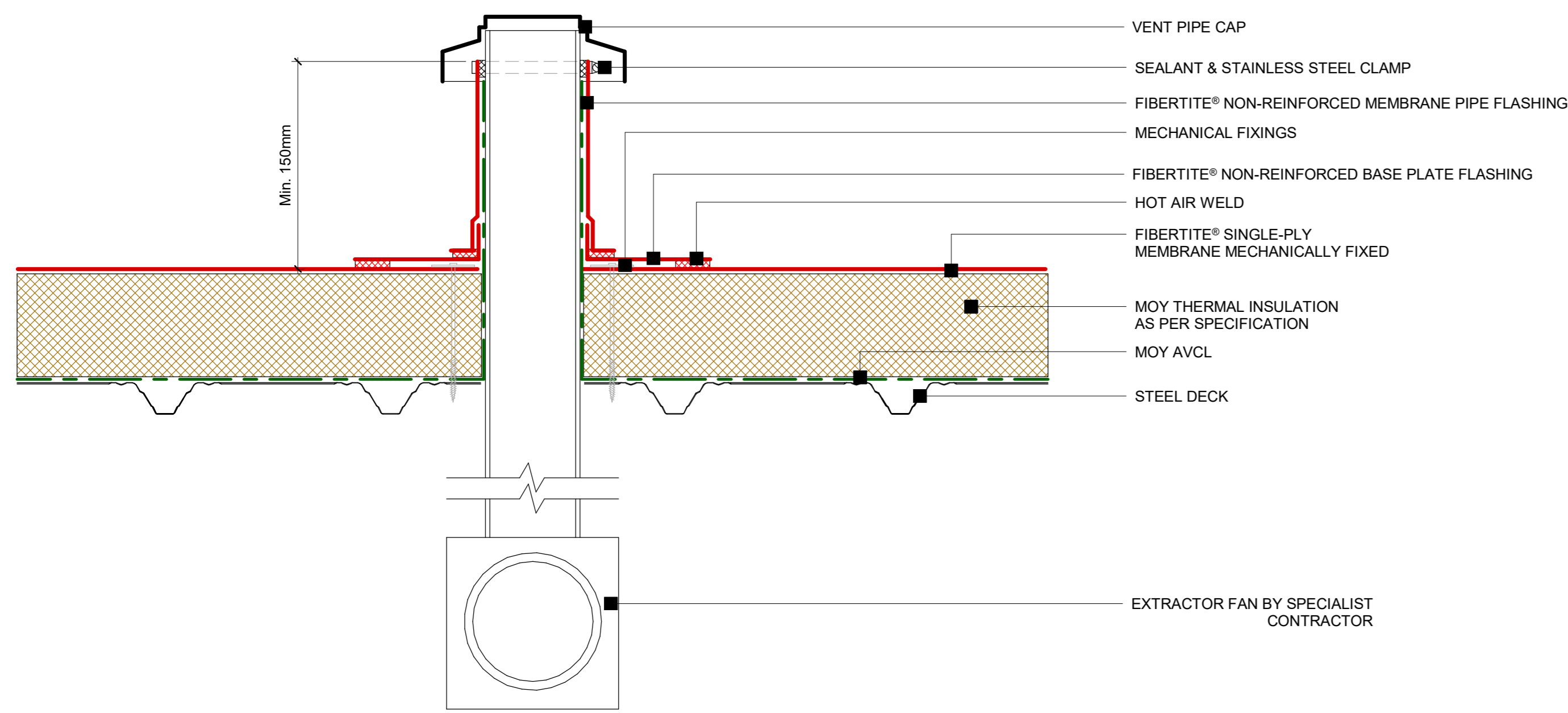
3 Fibertite® - Soil vent pipe detail (Site fabricated) 1 : 5
