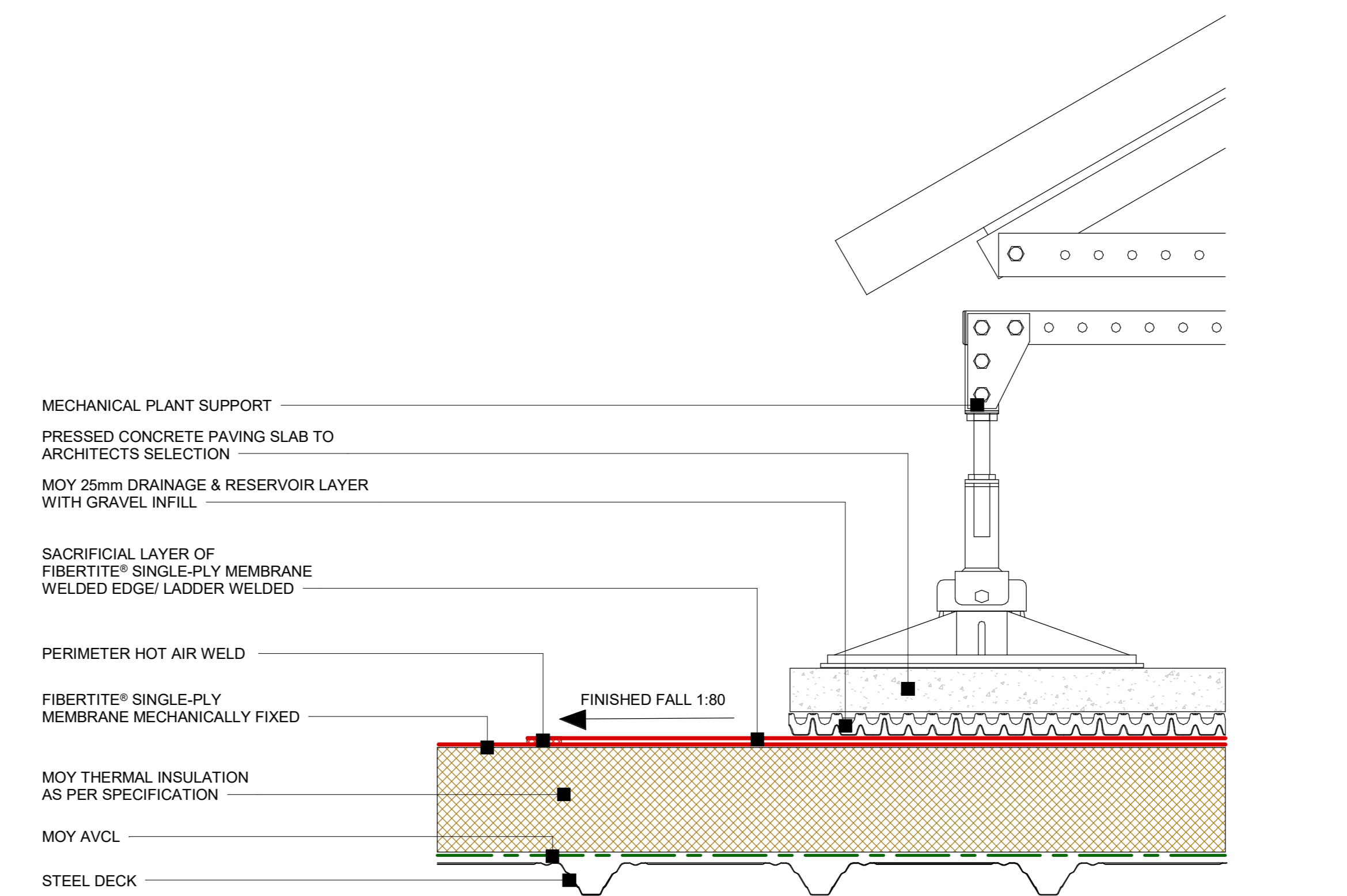
19 FiberTite® - Plant support detail 1 : 5
