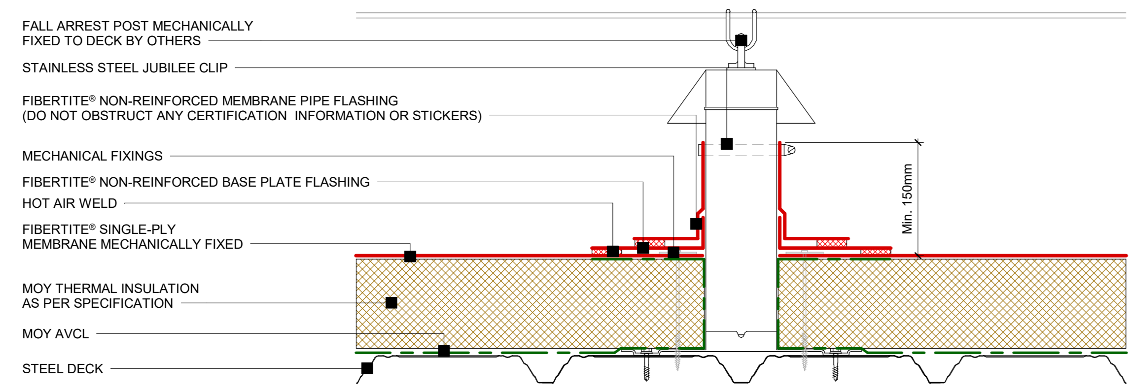
16 FiberTite® - Fall arrest detail 1 : 5
