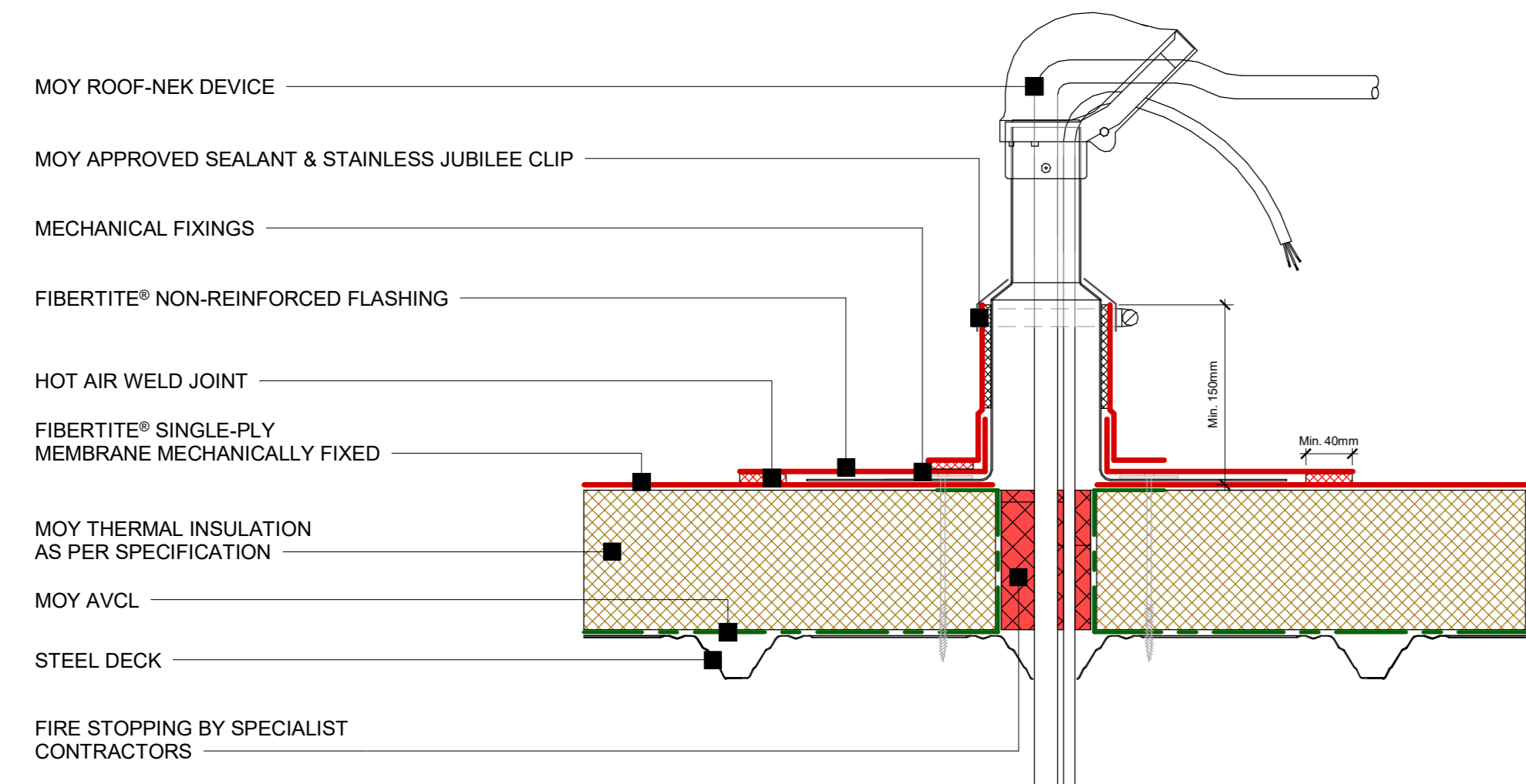
14 FiberTite® - RoofNek cable penetration detail 1 : 5
