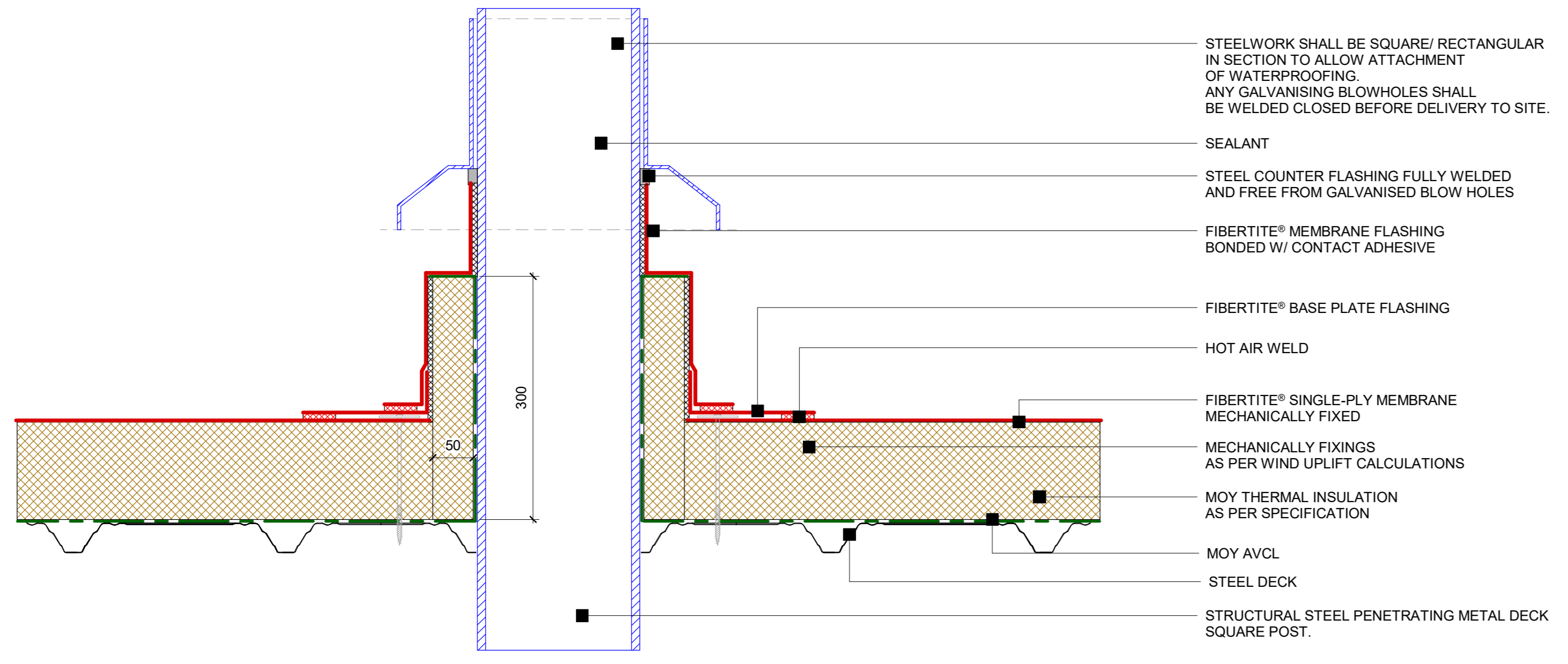
15 FiberTite® - Steel column penetration detail 1 : 5
